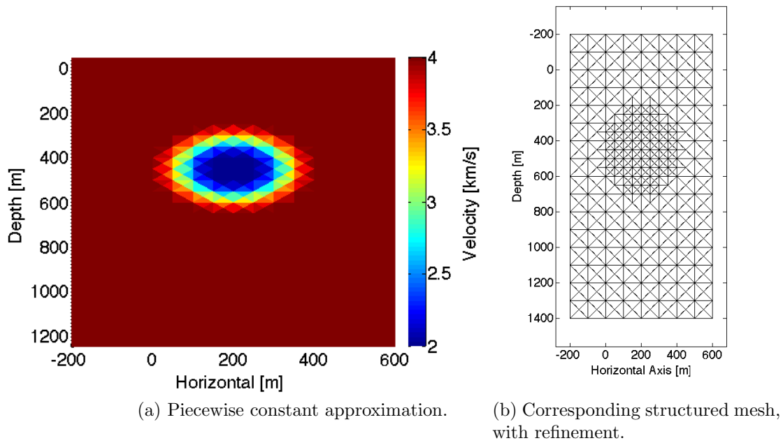
Figure 3.11 : Piecewise approximation of negative-lens velocity model and corresponding mesh, with mesh refinement.
