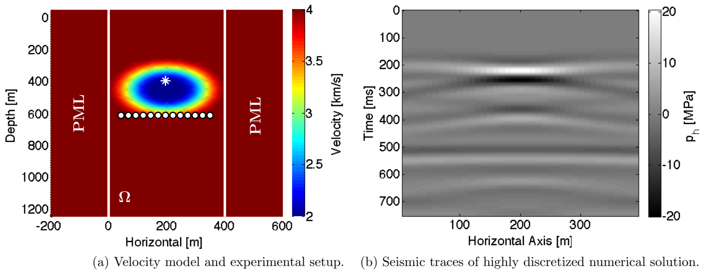
Figure 3.9 : Experimental setup and traces for negative-lens test case.
